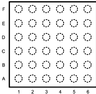
20202058 Top View (Bump Side Down) Order Number LM4937RL See NS Package Number RLA36LVA
