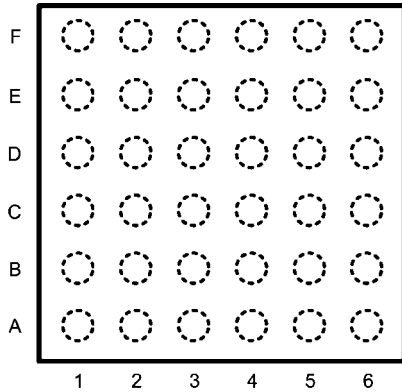
20202058 Top View (Bump Side Down) Order Number LM4937TL See NS Package Number TLA36LVA
