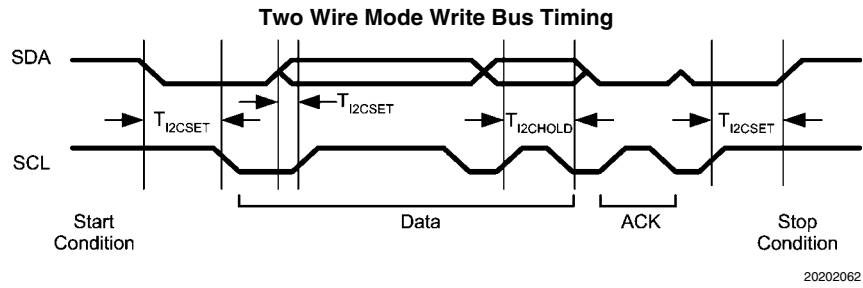
FIGURE 3. Two Wire Mode Write Bus
